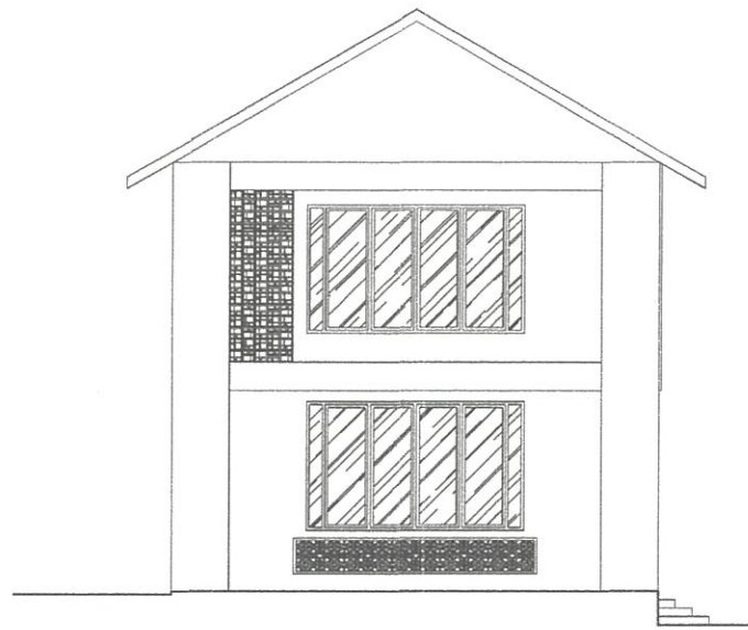
ARS TAMPAK SAMPING KIRI Scale 1:100
